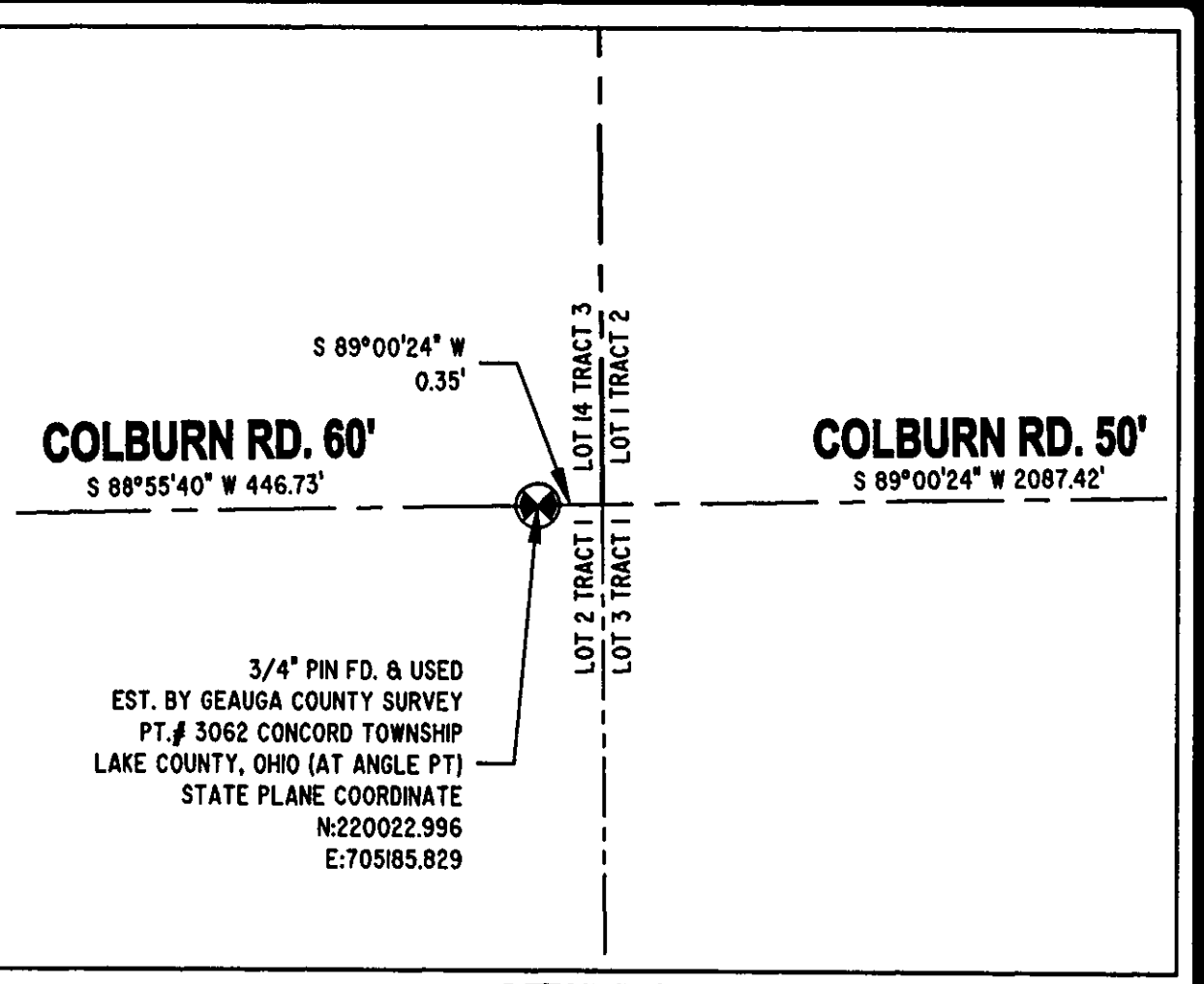
DETAIL "A": SCALE 1" = 1'
